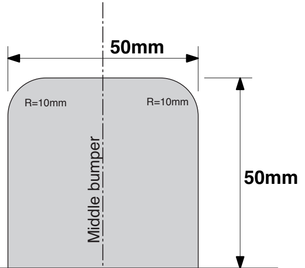
Underside bumper
